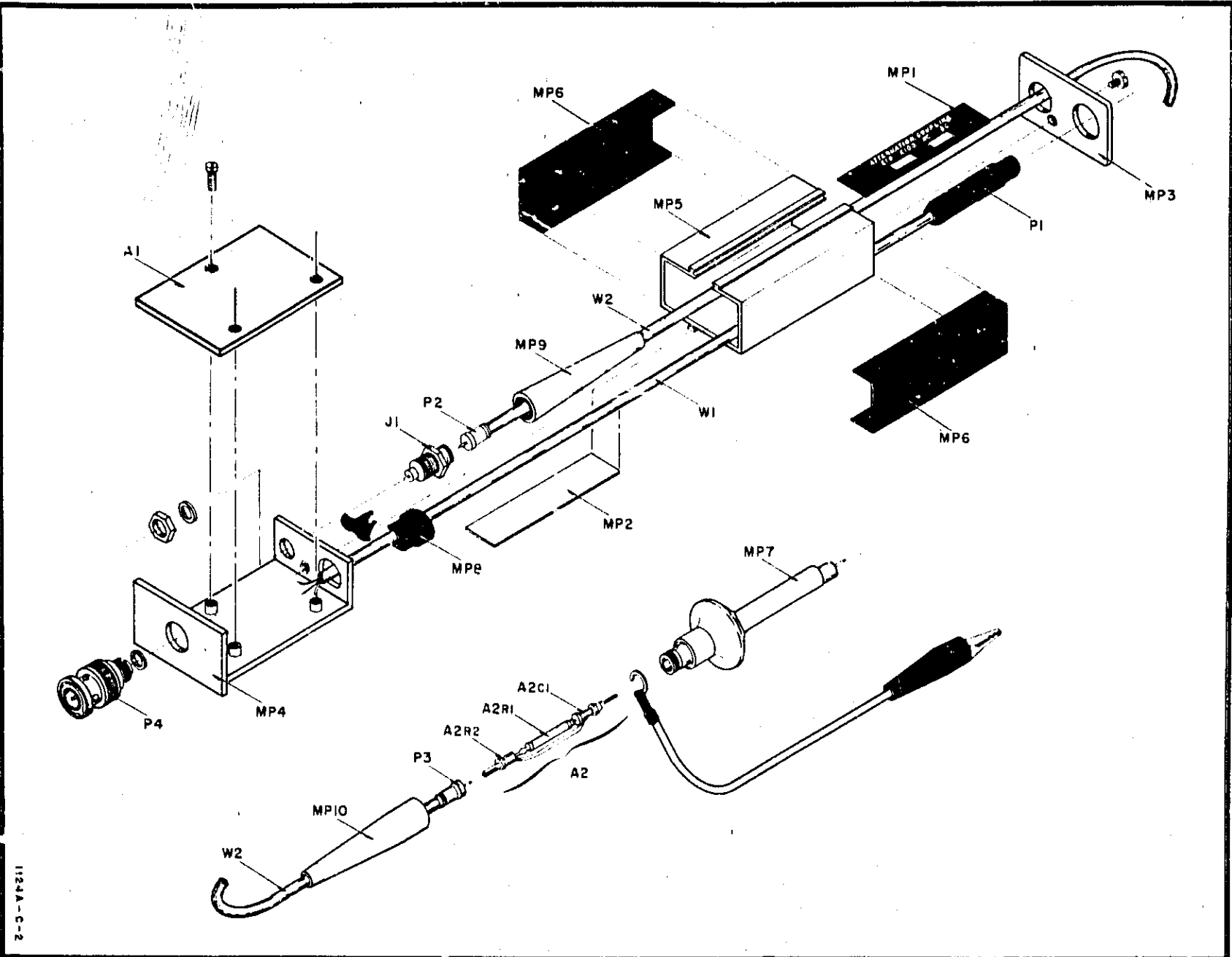
Figure 4. Model 1124A Exploded View
